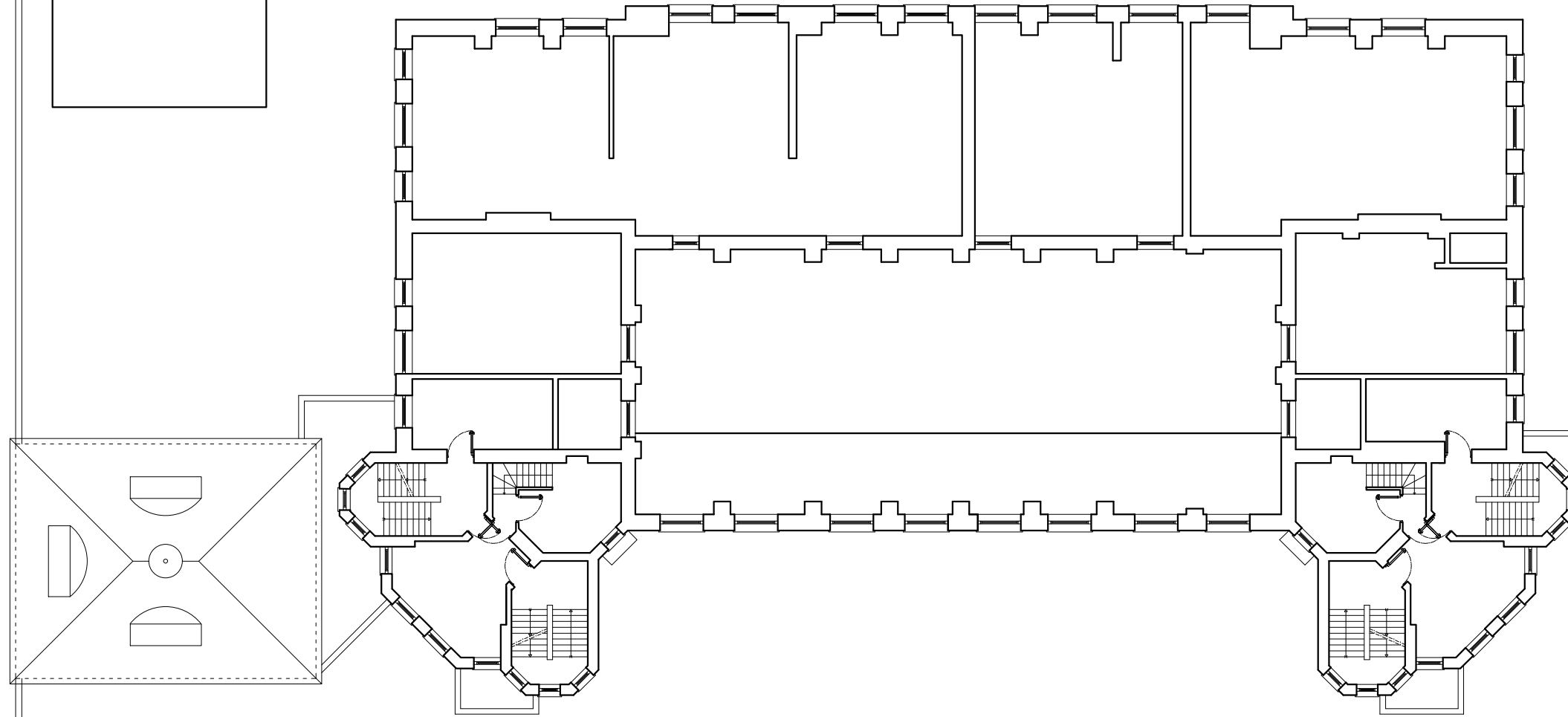
EXISTING GROUND FLOOR MEZZANINE PLAN SCALE: 1/200 @A3
